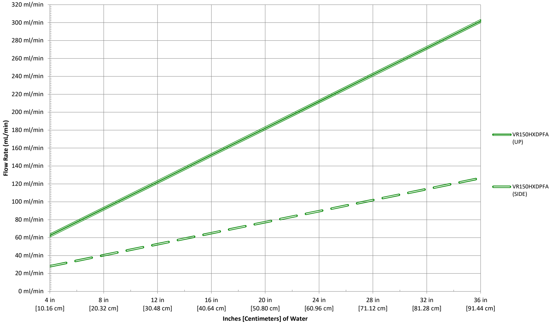
VR150HXDPFA Duck Drinker Flow Rates vs. Inches [Centimeters] of Water
