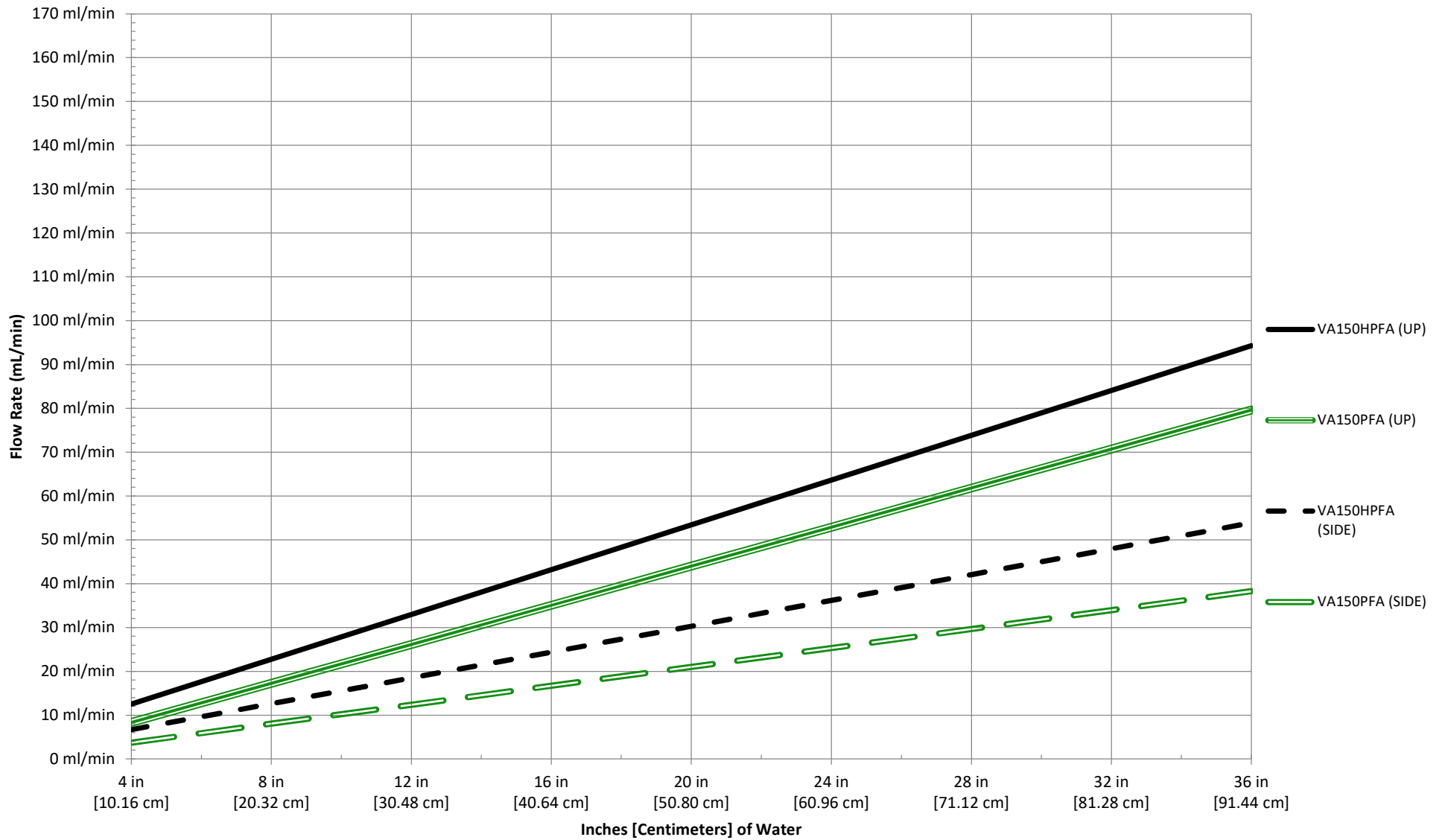
Aqua-V PFA Series Flow Rates vs. Inches [Centimeters] of Water
