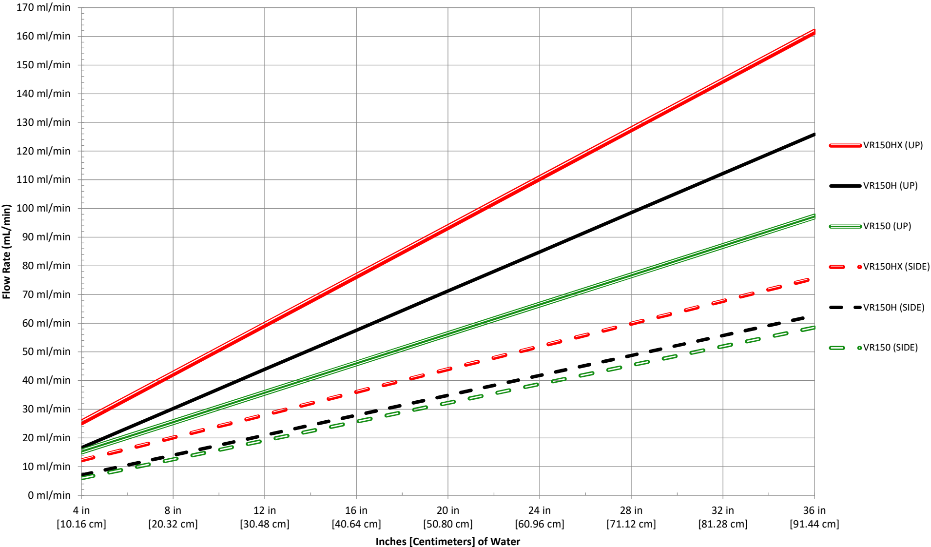
Roaster Series Flow Rates vs. Inches [Centimeters] of Water
