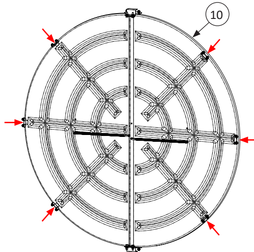
Magnet Locations
