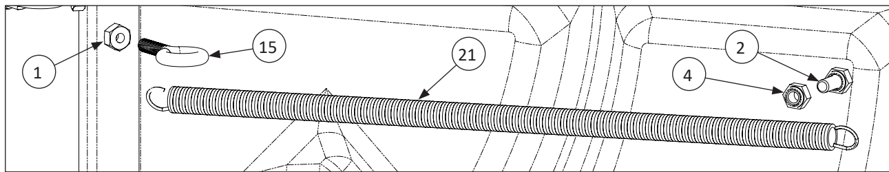
Enlarged Detail View: Damper Spring
