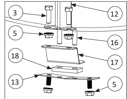
Enlarged Detail View: Damper Hardware
