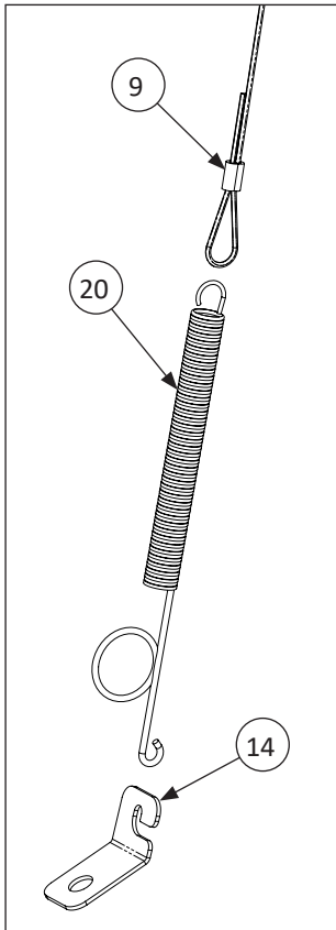
Enlarged Detail View: Damper Cable
