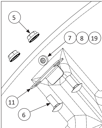
Enlarged Detail View: Magnets
