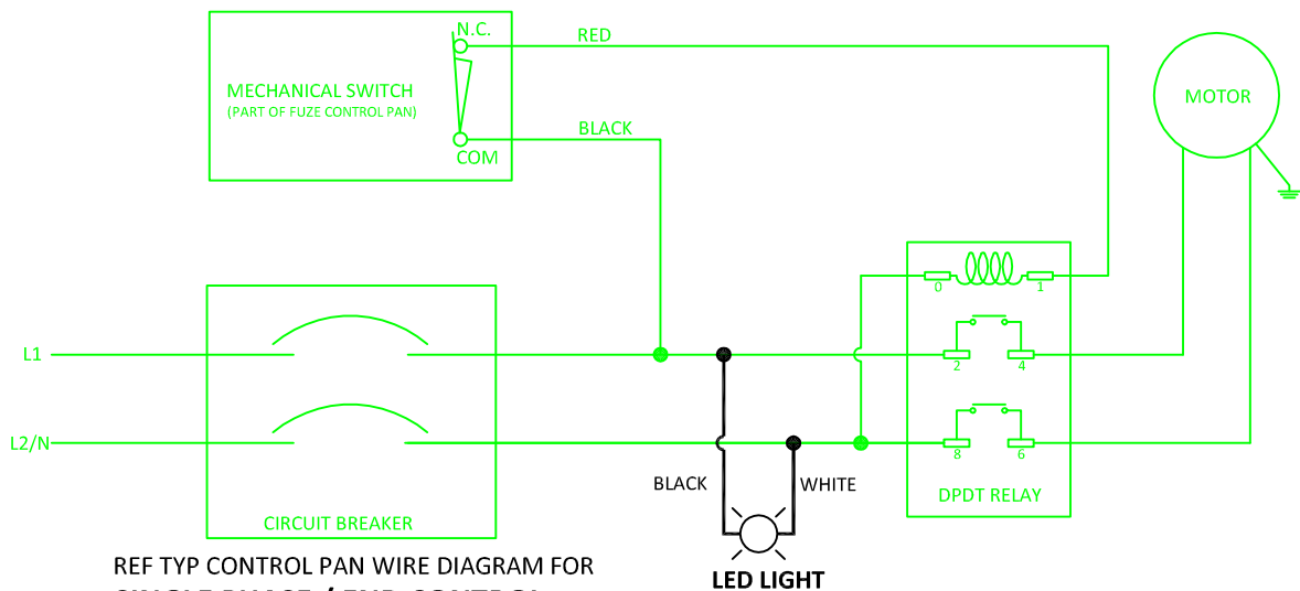
BASIC WIRE DIAGRAM FOR LED LIGHT WIRING MUST BE DONE BY LICENSED ELECTRICIAN. ALL LOCAL AREA CODES MUST BE FOLLOWED.
