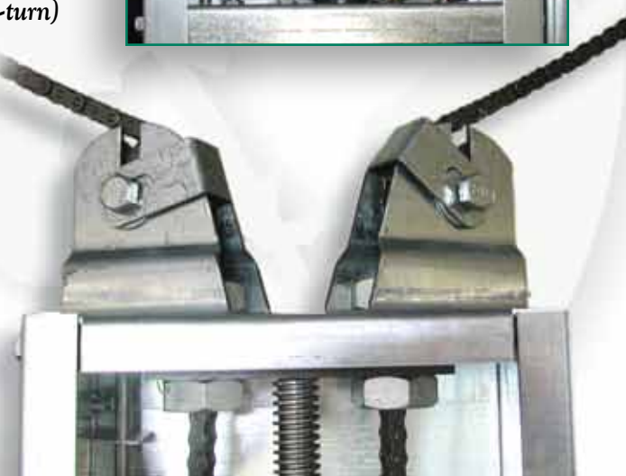
Right: Optional swivel chain and sprocket is also available.
