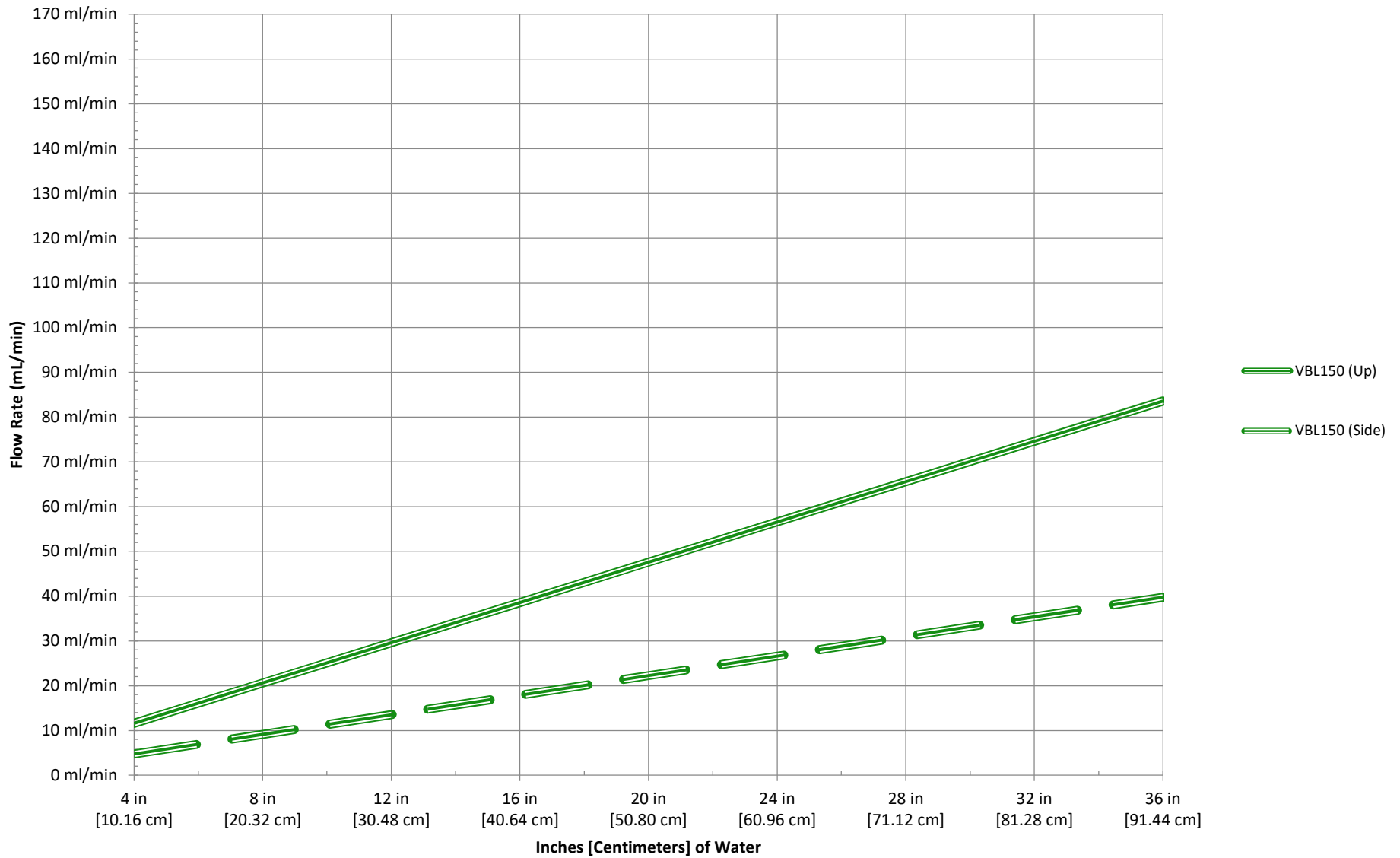
Broiler / Layer Drinker Flow Rates vs. Inches [Centimeters] of Water
