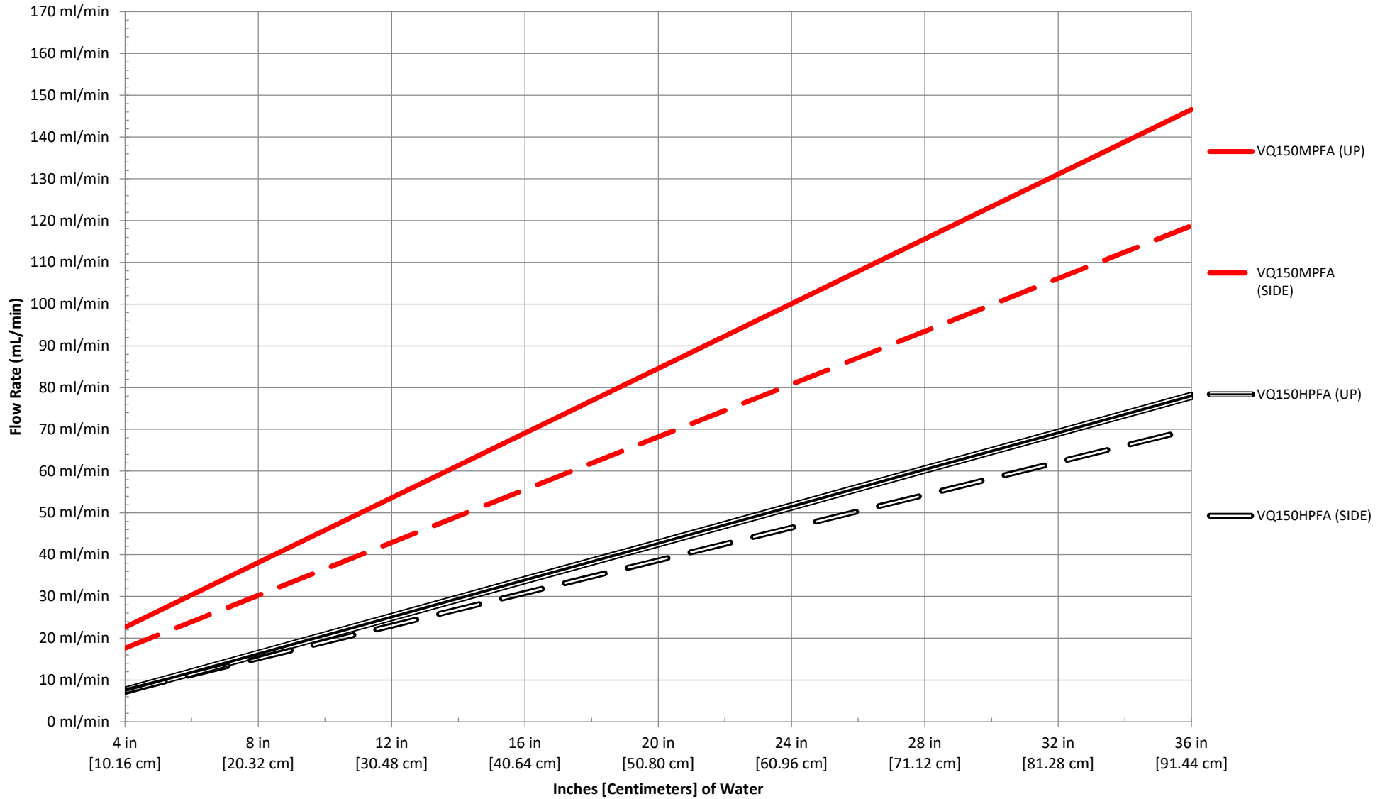
Quencher Series Flow Rates vs. Inches [Centimeters] of Water
