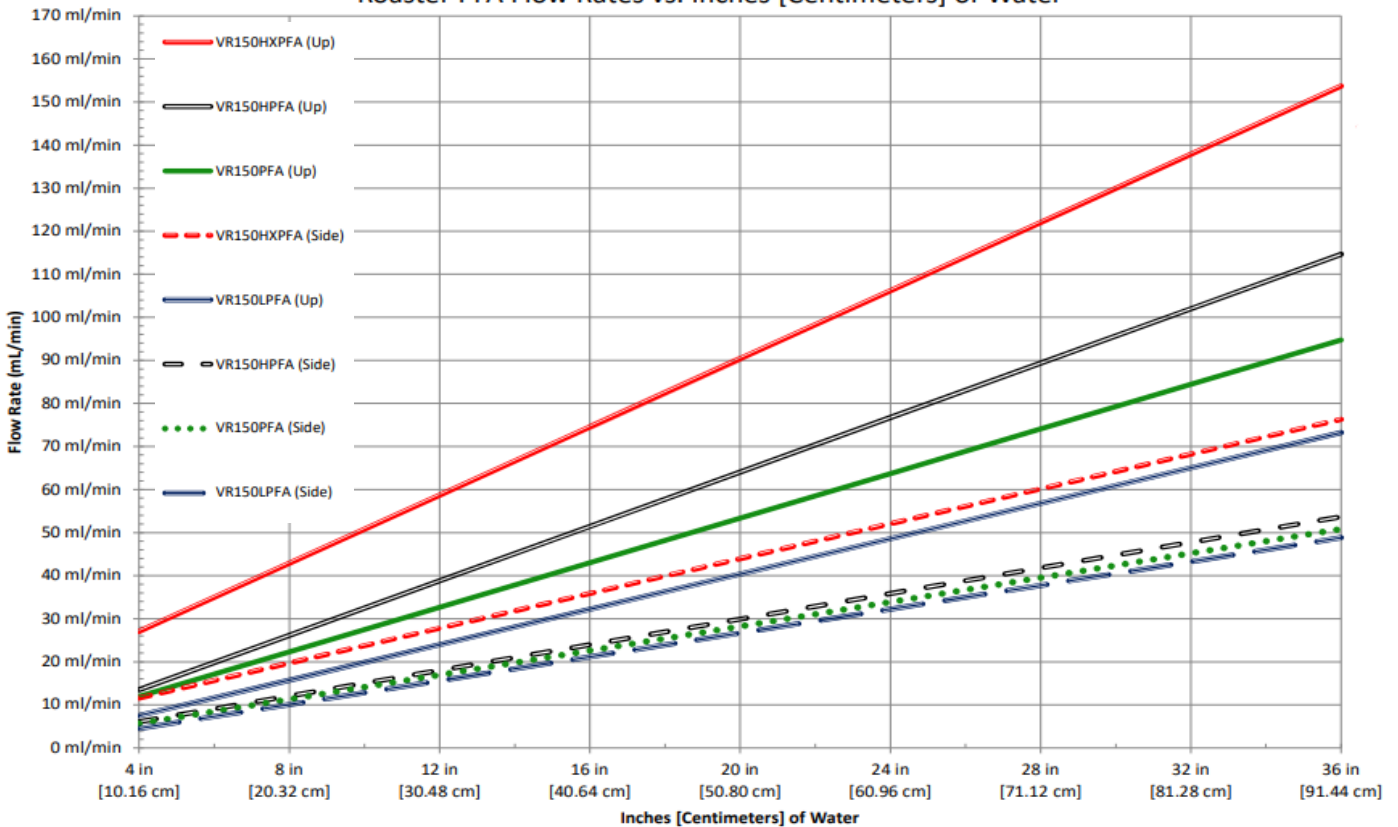
Roaster PFA Flow Rates vs. Inches [Centimeters] of Water
