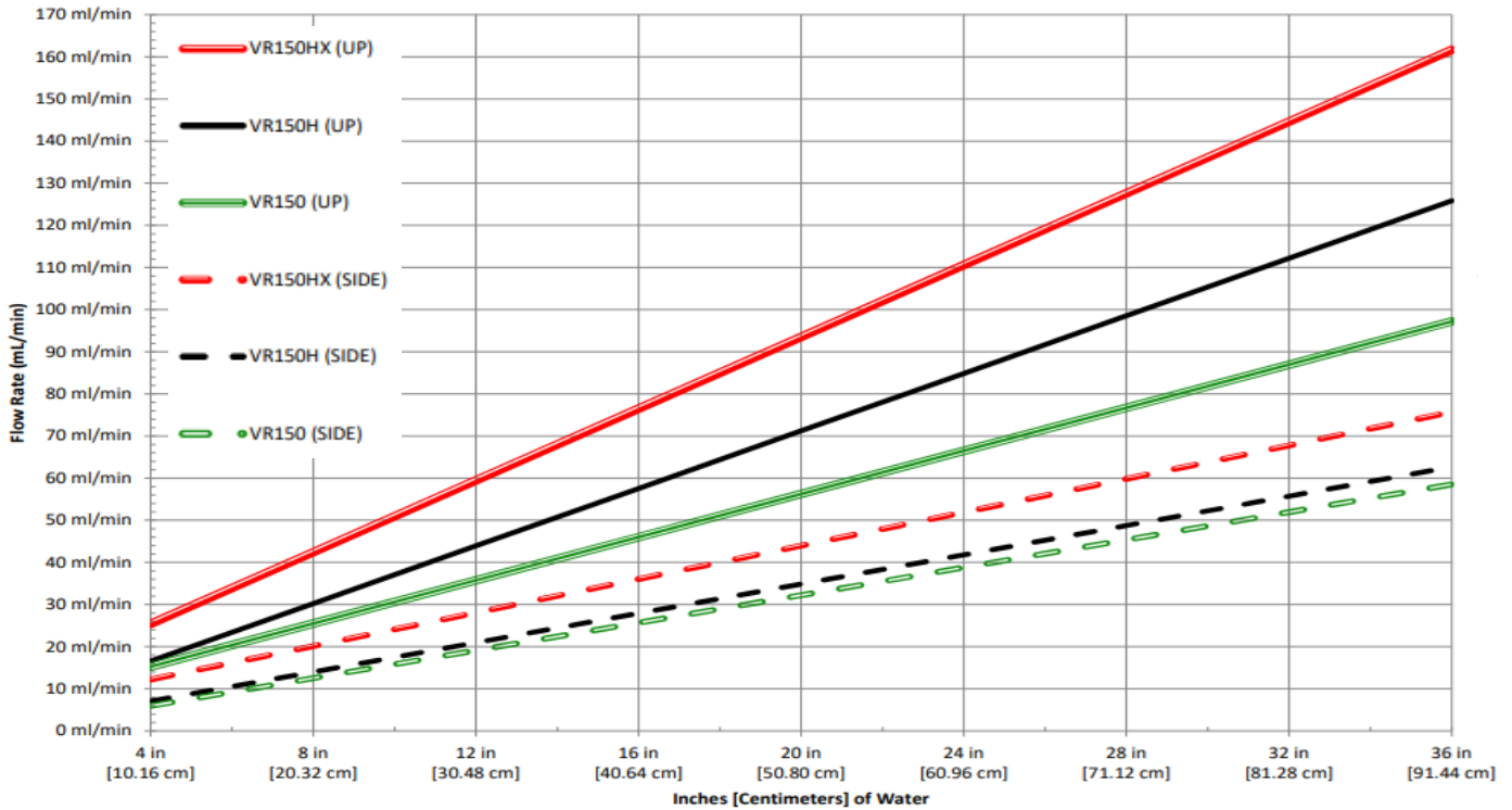
Roaster PFA Flow Rates vs. Inches [Centimeters] of Water
